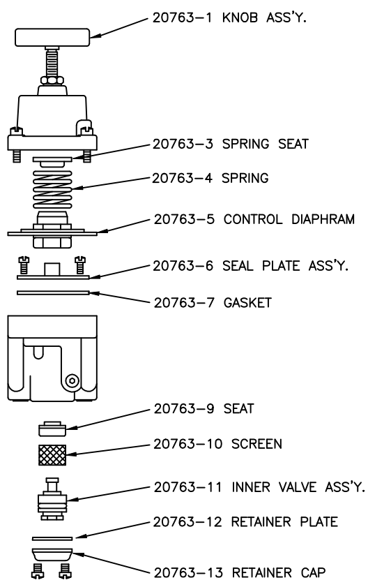
3/8"AIRBAG REGULATOR 20763
